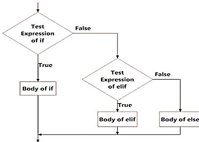
Fig: Operation of if – elif - else statement
